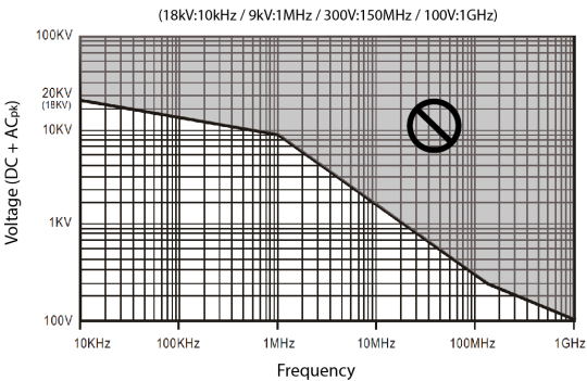
Figure 5: Voltage Derating Curve
