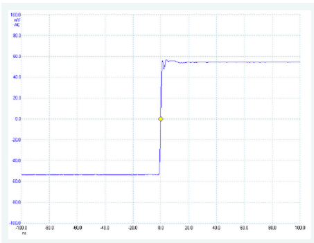
Figure 4: Compensation correcte
