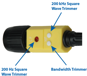
Figure 2: Frequency Compensation Trimmers
